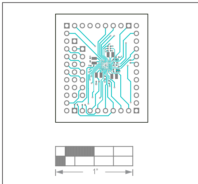
MAX20345 EV Kit PCB—Top Layer
