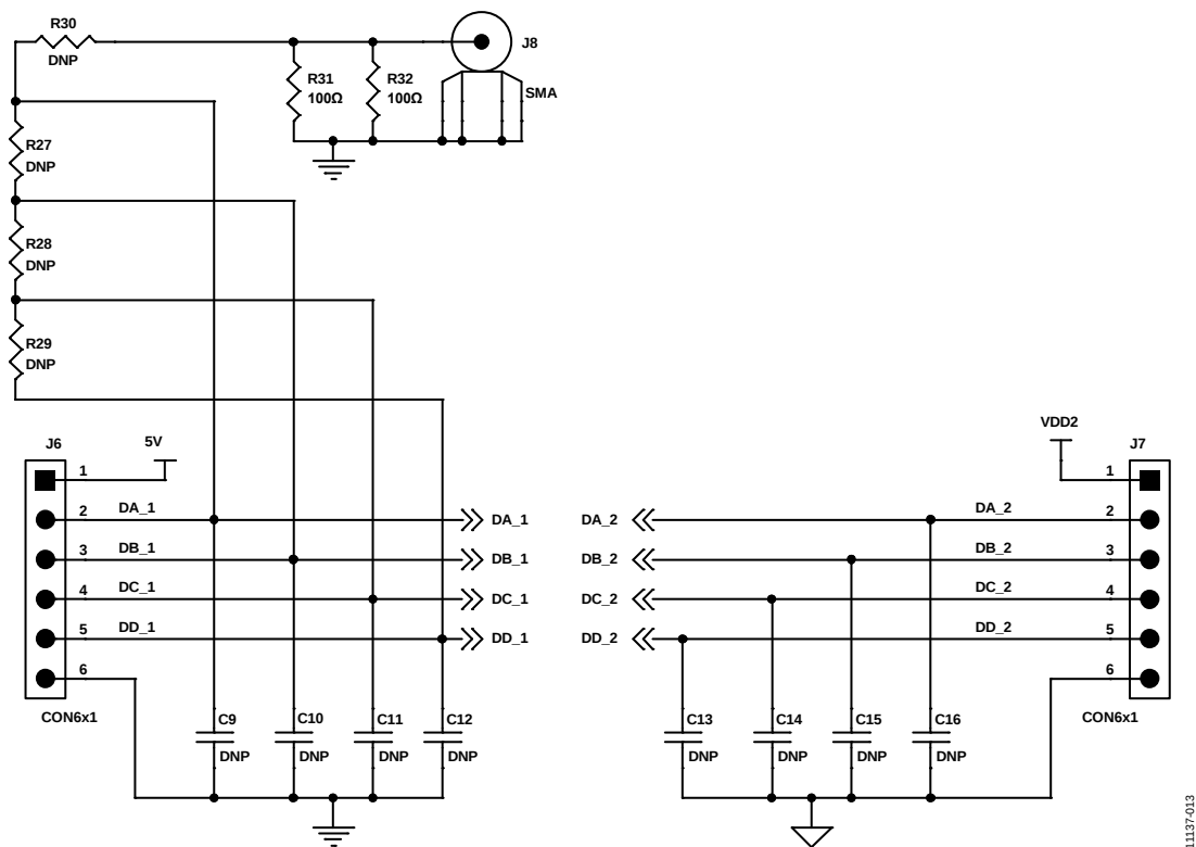
Figure 13. Evaluation Board Schematic, Page 2
