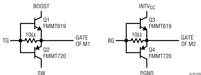
Figure 5. Optional External Gate Driver
