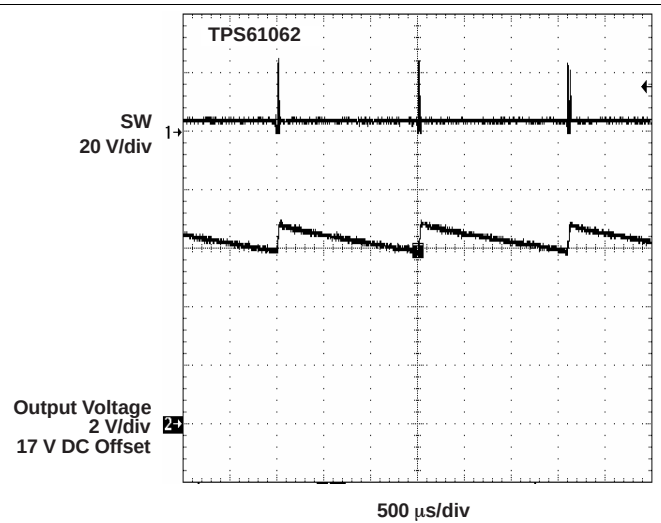
Figure 15. Overvoltage Protection
