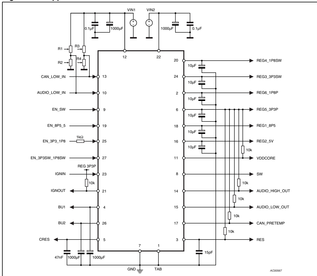
Figure 3. Application circuit
