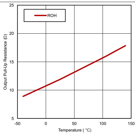
Figure 12. Output Pullup Resistance vs Temperature
