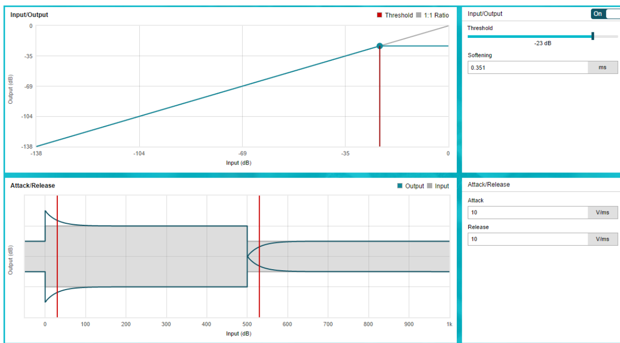
Figure 8. Full-Band AGL
