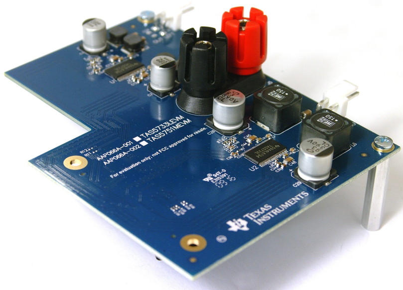
Figure 9. TAS5733LEVM
