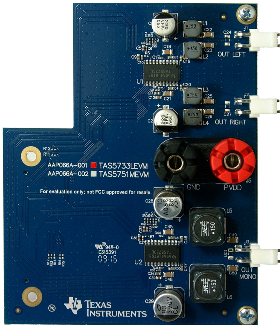
Figure 1. TAS5733L Evaluation Board
