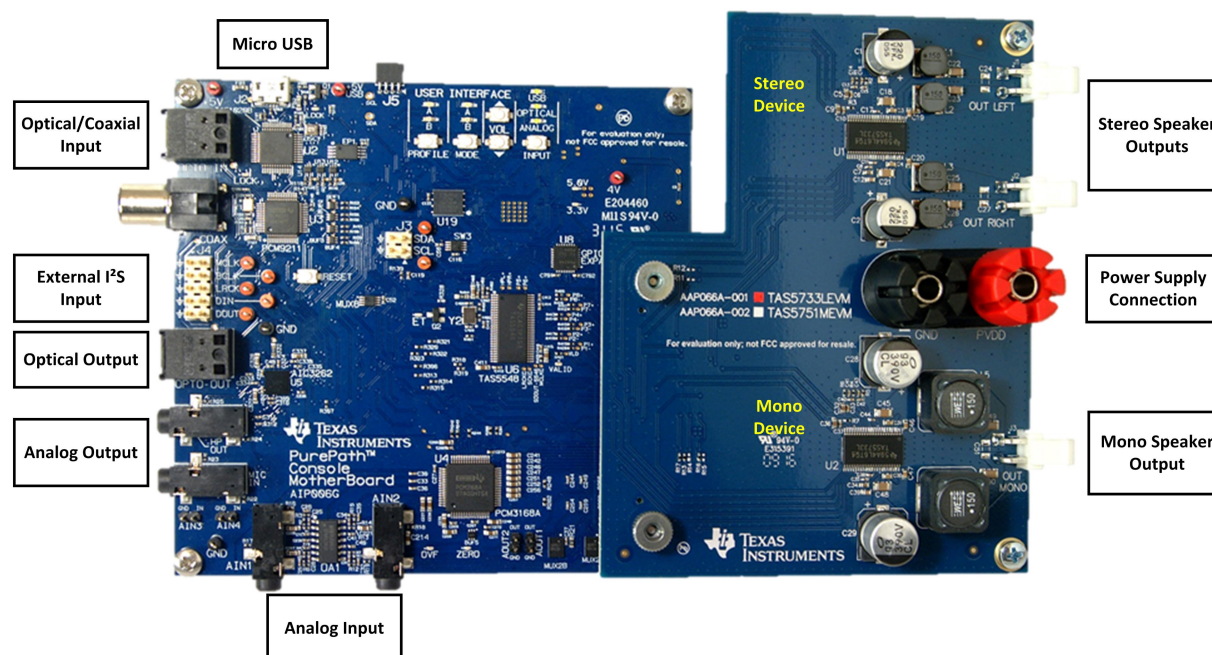
Figure 2. Evaluation Module and PurePath Console Motherboard Connection
