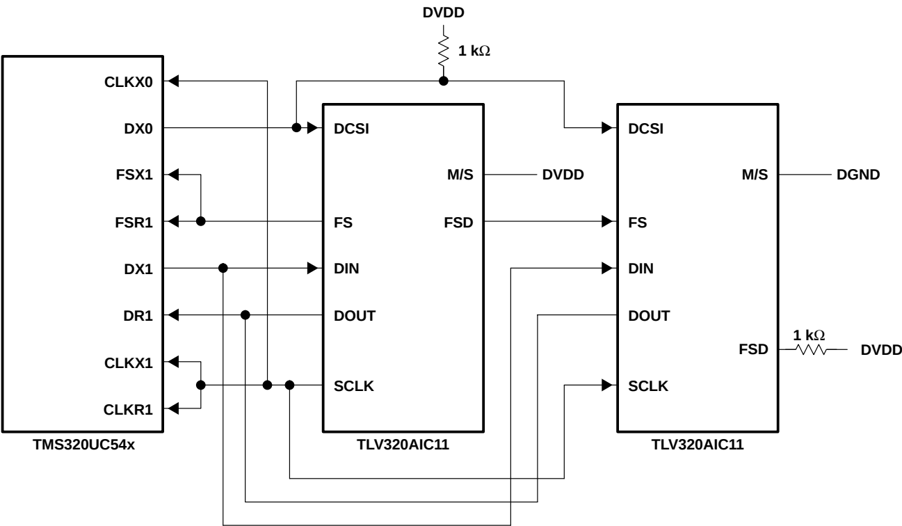
Figure 3–8. Direct Configuration
