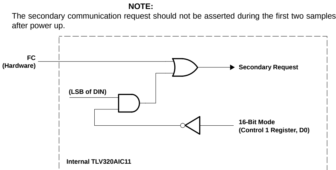
Figure 3–2. Hardware and Software Secondary Communication Request
