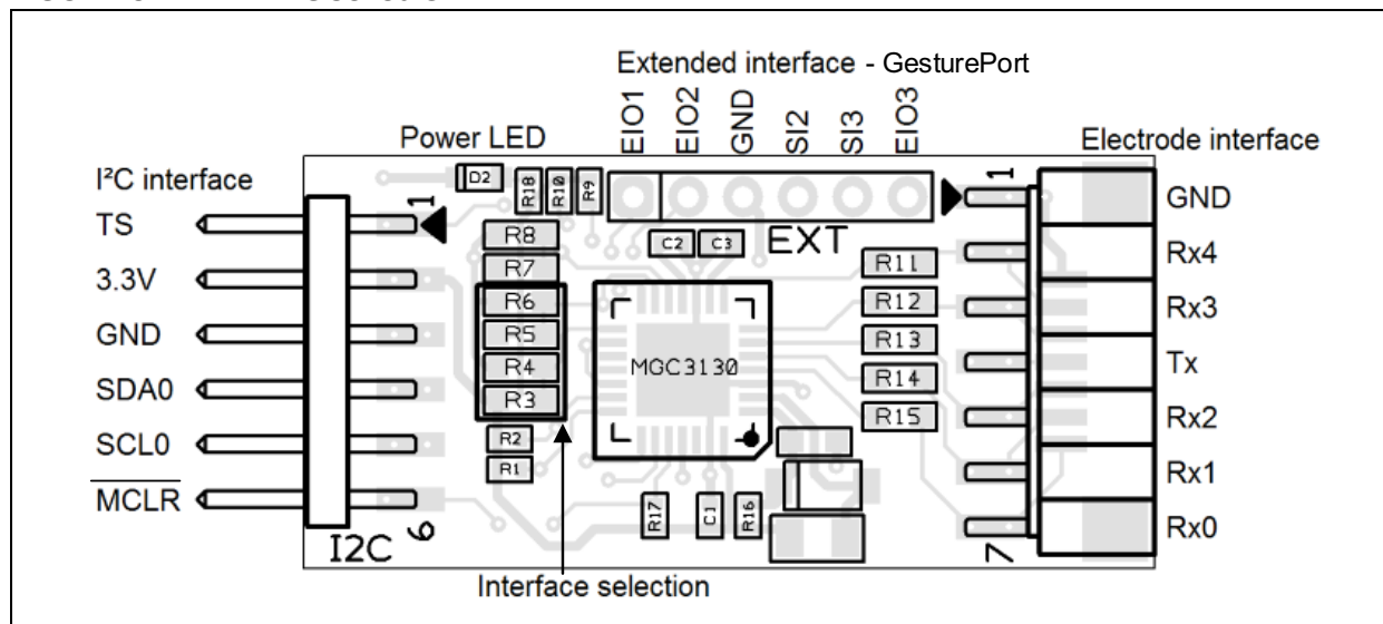
FIGURE 3-2: MGC3130 UNIT
