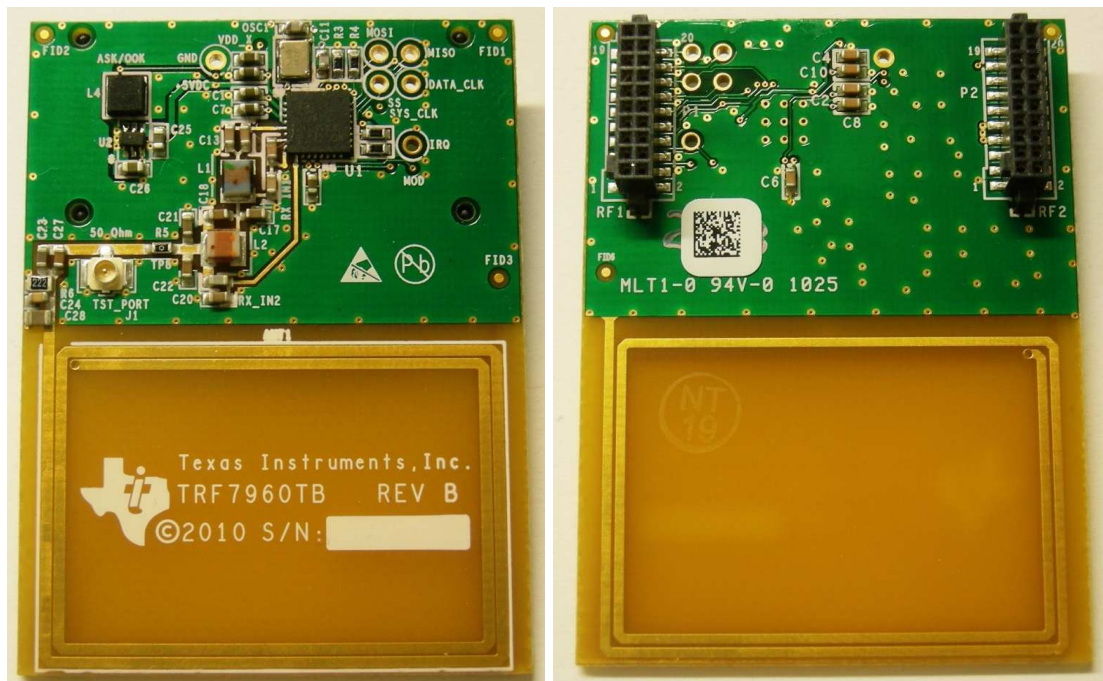
Figure 1. TRF7960TB Evaluation Module
