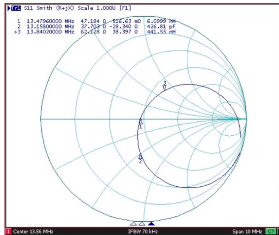
Figure 12. Higher Q Antenna Measurement Plots with Calculated Values ( Q \approx 20 )
