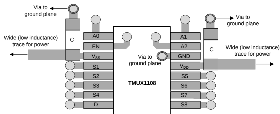
Figure 35. TMUX1108 Layout Example
