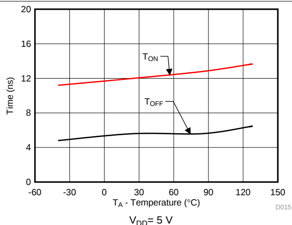
Figure 15. T_{ON} (EN) and T_{OFF} (EN) vs Temperature
