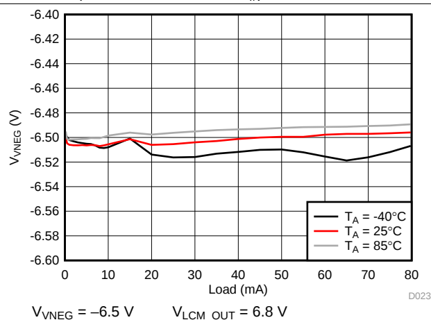
Figure 26. V_{VNEG} Load Regulation
