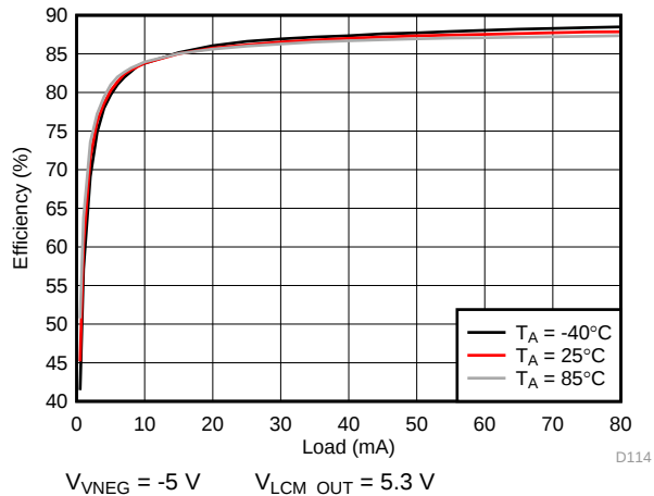
Figure 128. VNEG Efficiency
