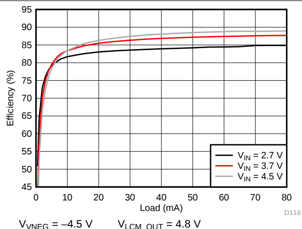
Figure 130. VNEG Efficiency
