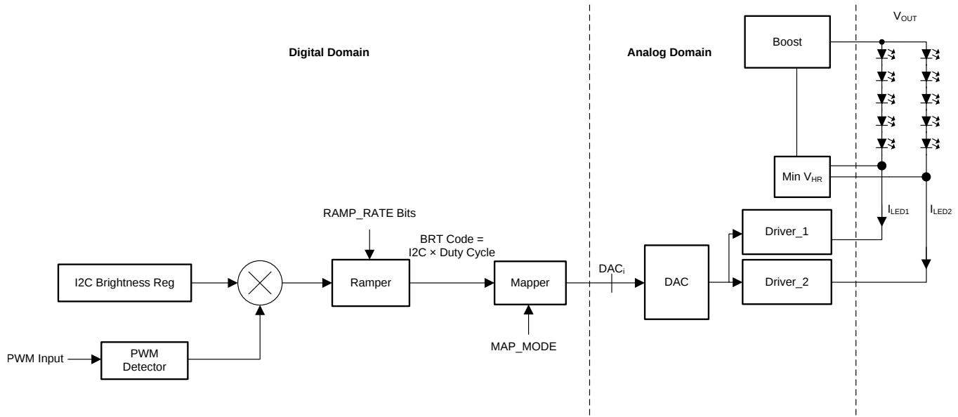
Figure 36. ( I^2C + PWM) Brightness Control, PWM Ramper Enabled
