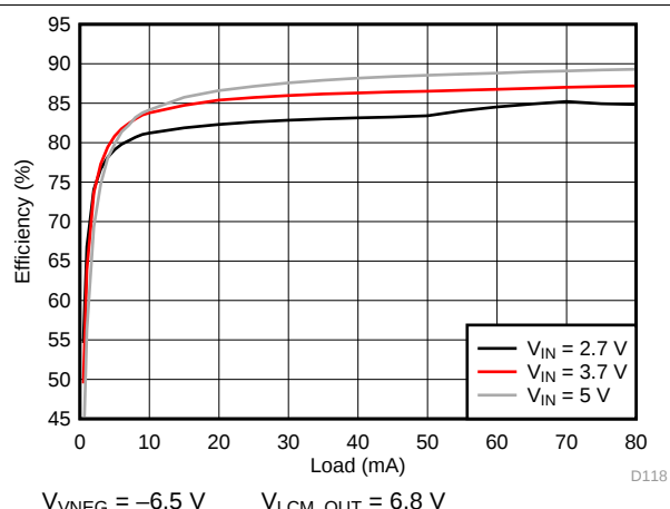
Figure 132. VNEG Efficiency
