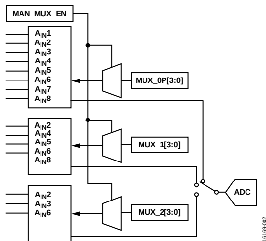
Figure 2. Manual Muxing Scheme for ADV7280A-M
