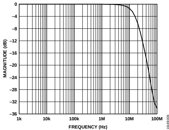
Figure 6. Antialiasing Filter Magnitude Response
