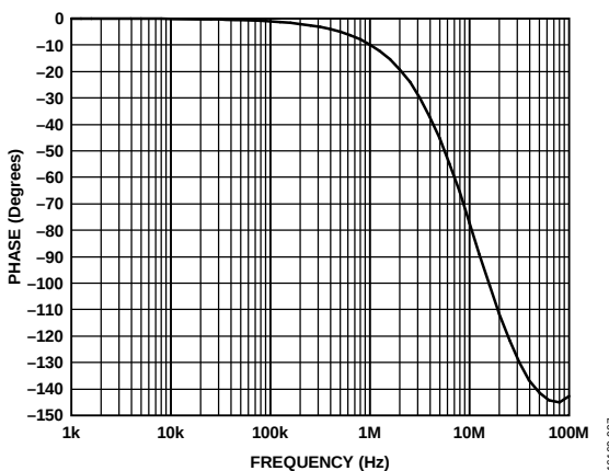
Figure 7. Antialiasing Filter Phase Response
