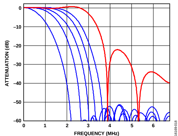
Figure 18. Chroma Shaping Filter Responses; Combined C Antialias, C Shaping Filter, and C Resampler
