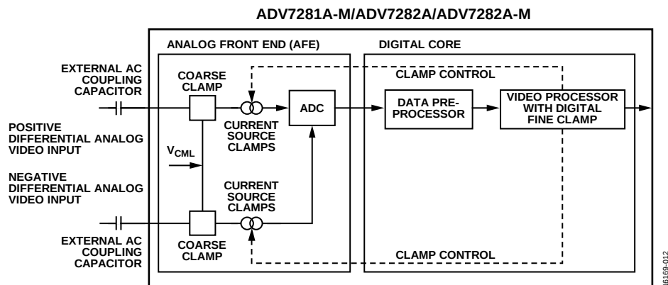
Figure 12. Differential Clamping Overview
