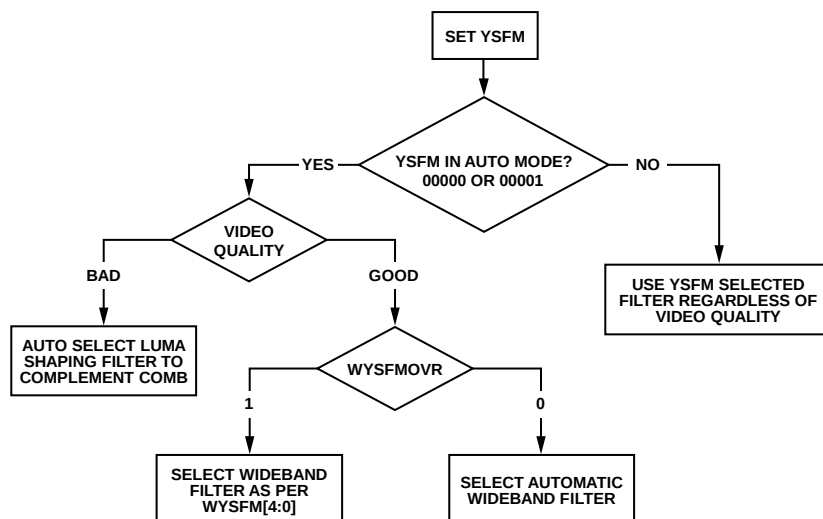
Figure 13. YSFM[4:0] and WYSFM[4:0] Control Flowchart
