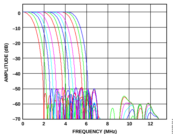
Figure 14. Combined Y Antialias, S-VHS Low-Pass Filter, and Y Resample Responses
