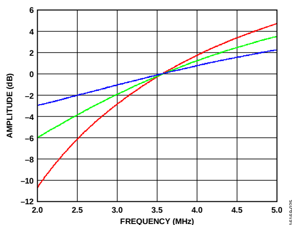
Figure 25. NTSC IF Filter Compensation (Zoomed Around f_{sc} )
