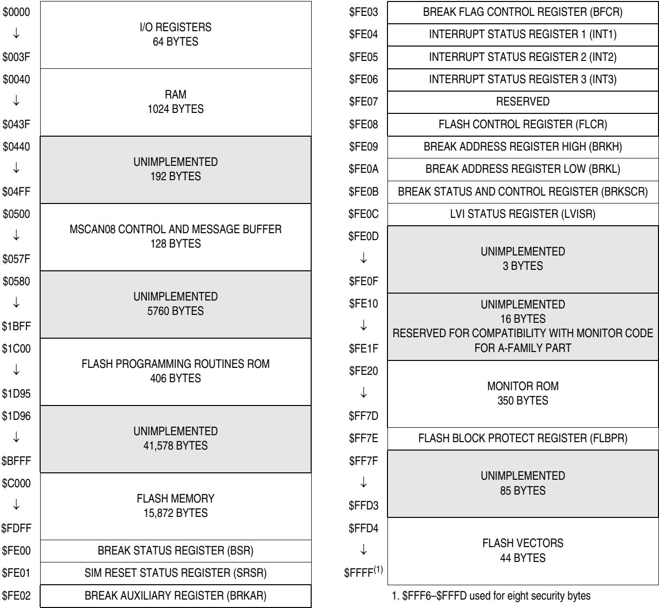
Figure 2-1. Memory Map
