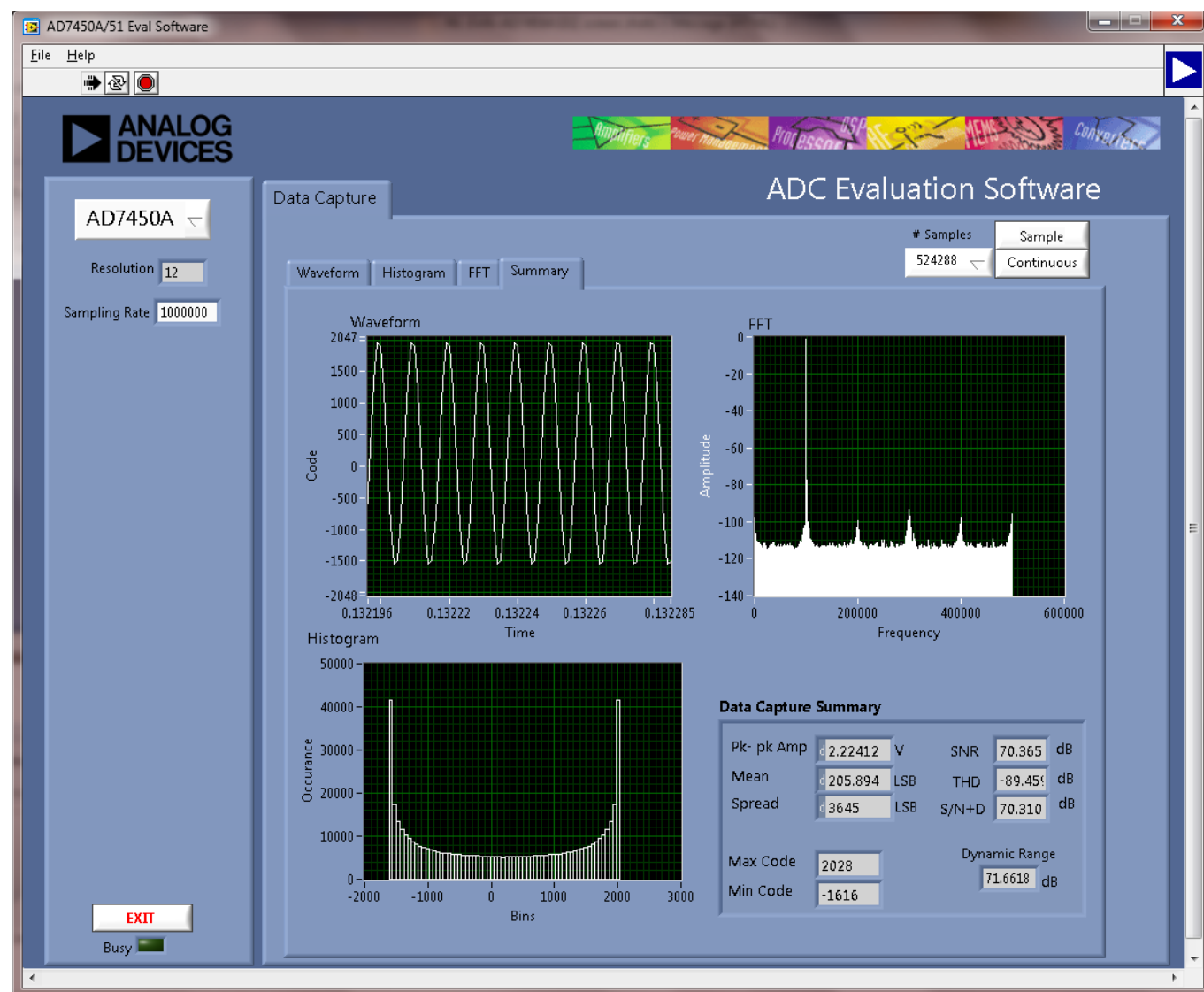
Figure 21. Summary Tab
