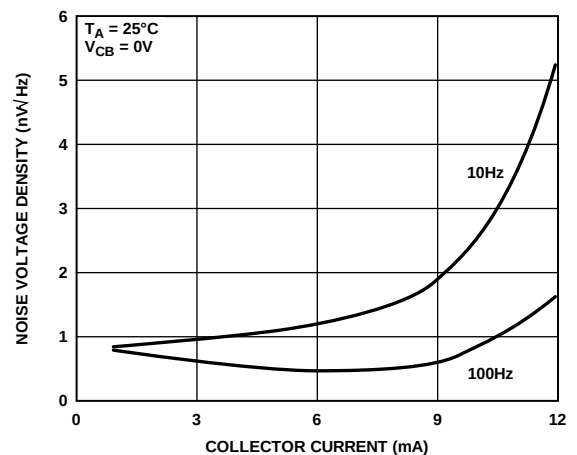
Figure 6. Noise Voltage Density vs. Collector Current
