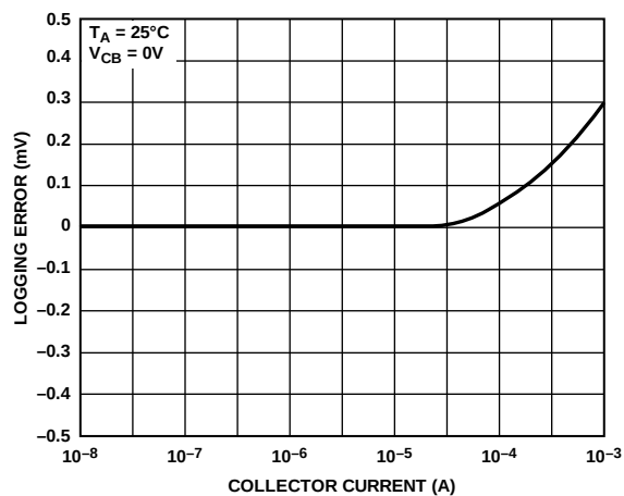
Figure 4. Emitter to Base Log Conformity
