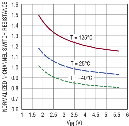
Normalized N-Channel Switch Resistance vs V_{IN}
