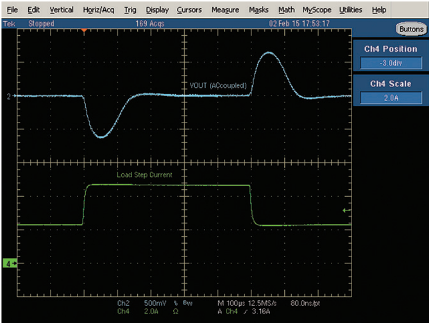
Figure 6. Load Transient Response ( V_{PORT} = 42.5V , 2.35A to 4.7A to 2.35A)
