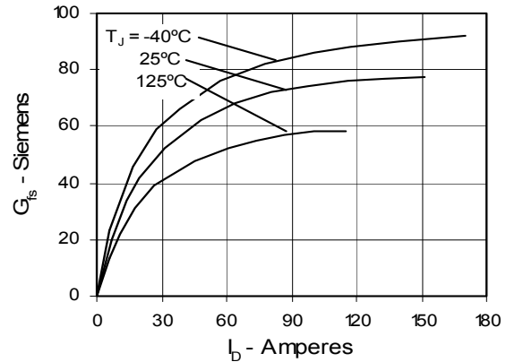
Fig. 8. Transconductance
