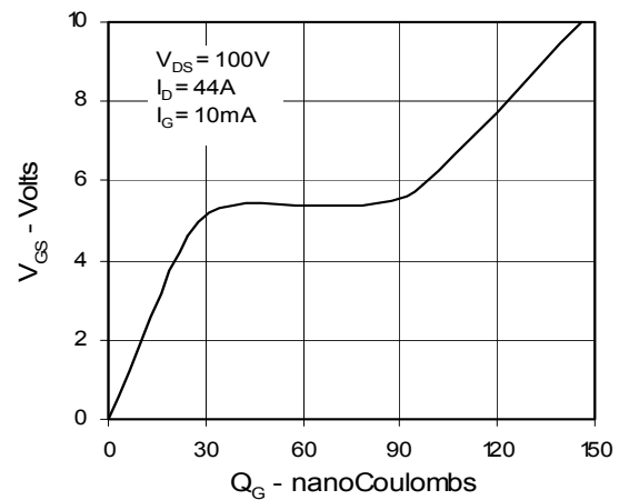
Fig. 10. Gate Charge
