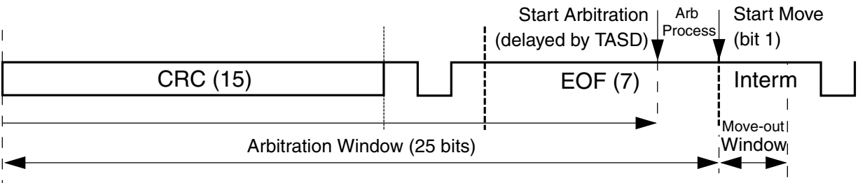
Figure 42-107. Arbitration and Move-Out Time Windows
