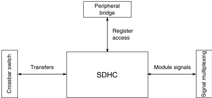
Figure 3-53. SDHC configuration
