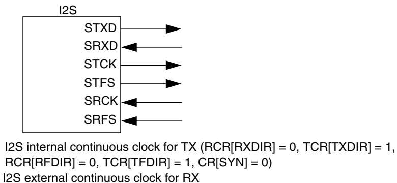
Figure 47-2. Asynchronous (SYN = 0) I2S configurations—continuous clock
