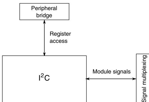
Figure 3-51. I2C configuration
