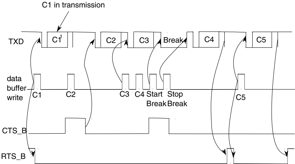
Figure 45-219. Transmitter RTS and CTS timing diagram
