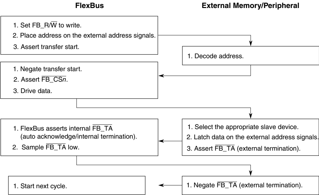
Figure 29-28. Write-Cycle Flowchart
