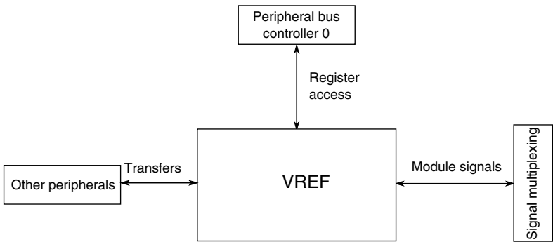
Figure 3-40. VREF configuration
