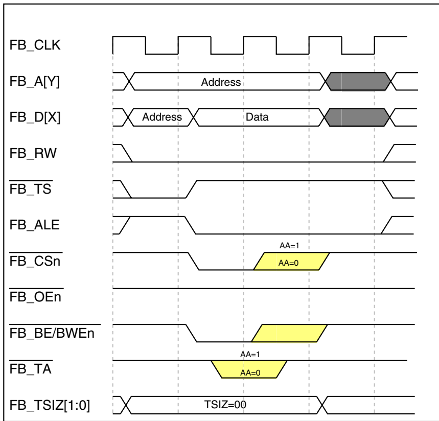
Figure 29-35. Longword-Write Transfer
