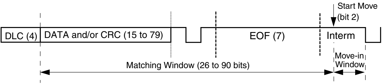
Figure 42-106. Matching and Move-In Time Windows
