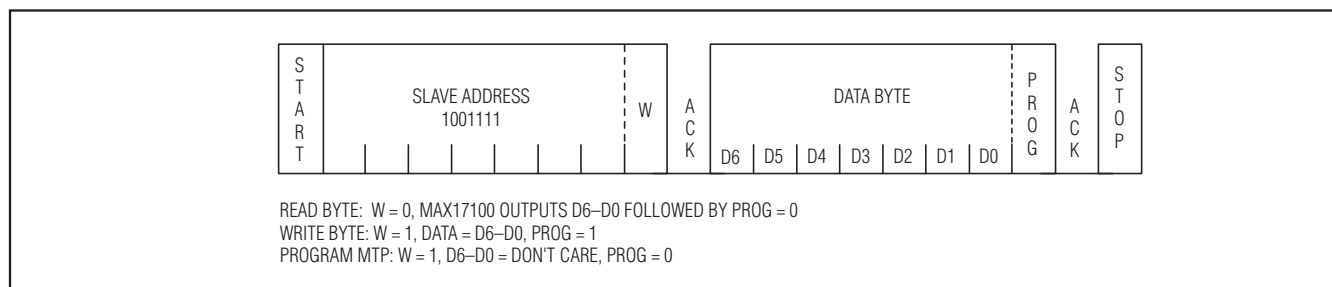
Figure 14. Serial Slave Address and Data Byte
