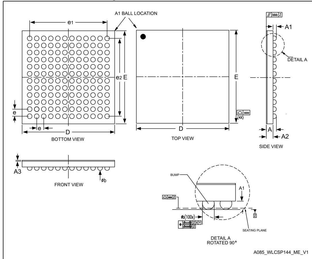
Figure 75. WLCSP144 outline
