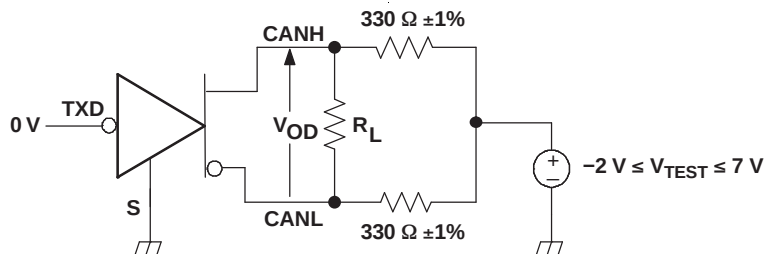
Figure 3. Driver V_{OD} Test Circuit
