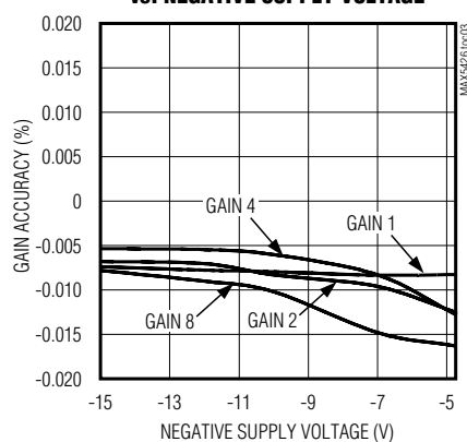
MAX5426A GAIN ACCURACY vs. NEGATIVE SUPPLY VOLTAGE
