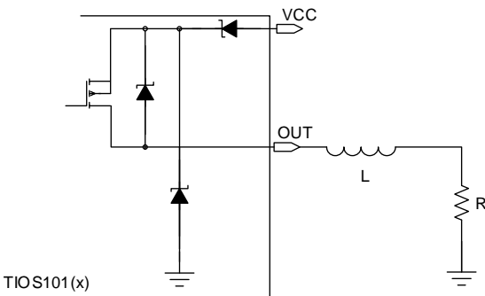
Figure 15. PNP Mode
