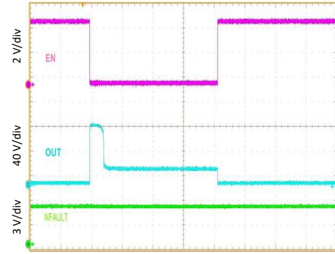
Figure 24. OUT Driving, Low Side Mode Time 10 ms/div 1.5-H Induct With = 100 Ω or R SET = OPEN
