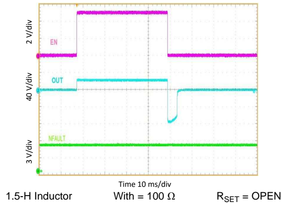
Figure 25. OUT Driving, High Side Mode 1.5-H Inductor Time 10 ms/div With = 100 Ω R SET = OPEN
