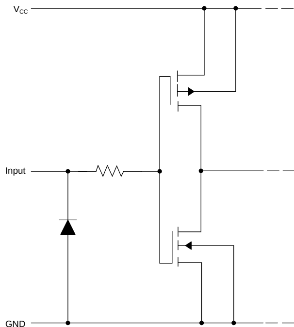
Figure 8. Equivalent of Each Input (A, G, or \overline{G} ) Schematic
