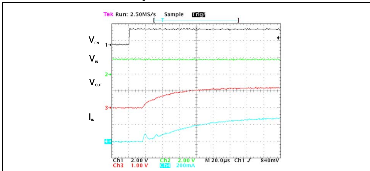
Figure 4. Soft-start function
