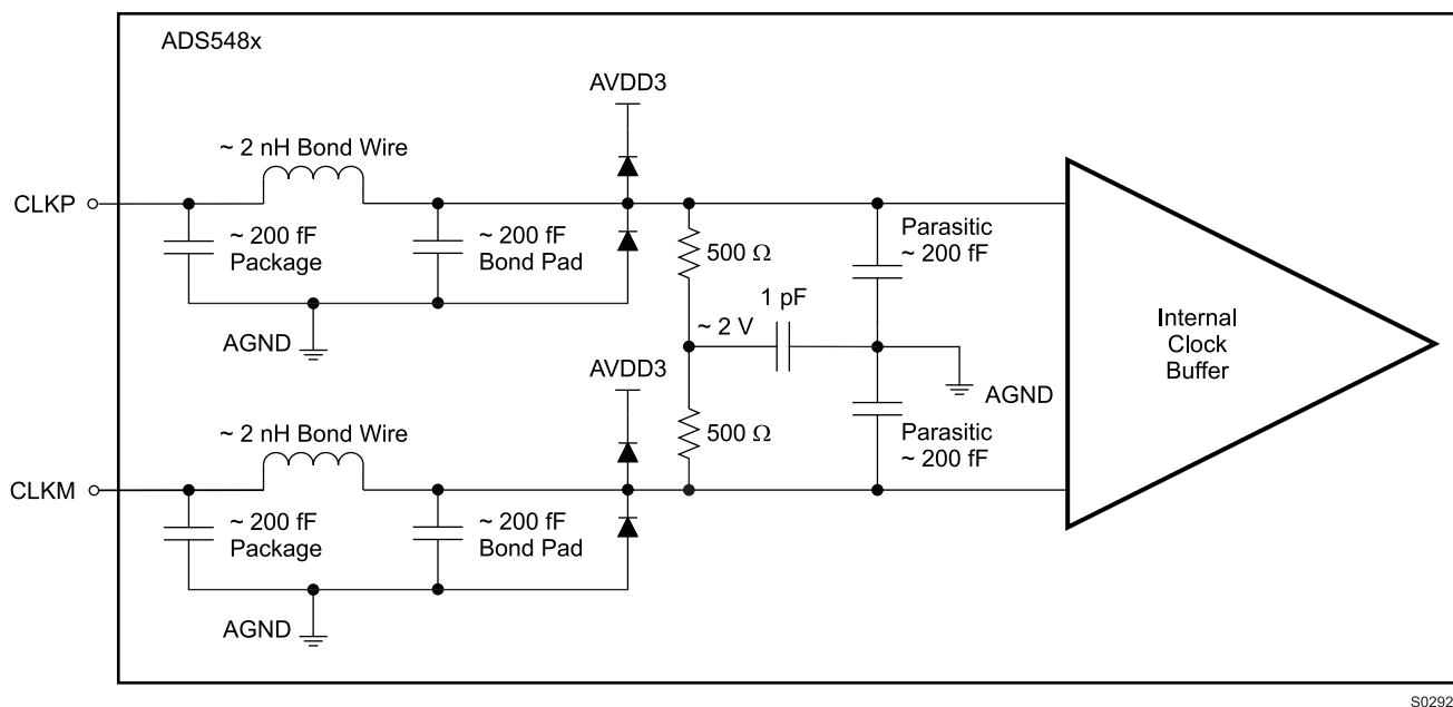
Figure 37. Clock Input Circuit
