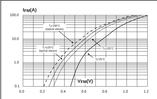
Figure 7. Forward voltage drop vs. forward current (typical values, per diode)
