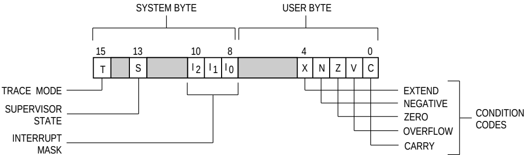
Figure 2-4. Status Register
