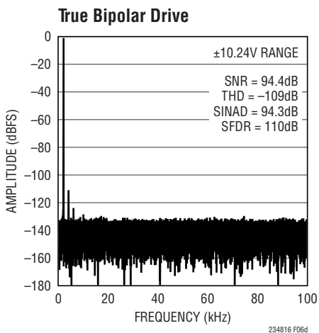
Figure 6d. IN^+ = -1\text{dBFS} 2kHz True Bipolar Sine, IN^- = 0\text{V} , 32k Point FFT, f_{\text{SAMPL}} = 200\text{kpsps} . Circuit Shown in Figure 6a with LT1469 Amplifiers, R_{\text{FILT}} = 49.9\Omega , C_{\text{FILT}} = 1000\text{pF}
