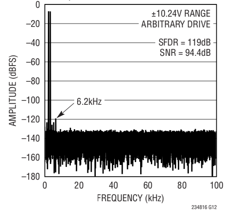
32k Point Arbitrary Two-Tone FFT f_{SMPL} = 200\text{kHz} , IN^+ = -7\text{dBFS } 2\text{kHz} Sine, IN^- = -7\text{dBFS } 3.1\text{kHz} Sine
