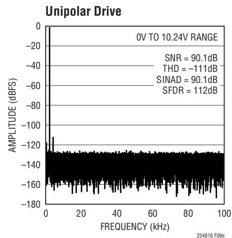
Figure 6e. IN^+ = -1\text{dBFS} 2kHz Unipolar Sine, IN^- = 0\text{V} , 32k Point FFT, f_{\text{SAMPL}} = 200\text{kpsps} . Circuit Shown in Figure 6a with LT1469 Amplifiers, R_{\text{FILT}} = 49.9\Omega , C_{\text{FILT}} = 1000\text{pF}
