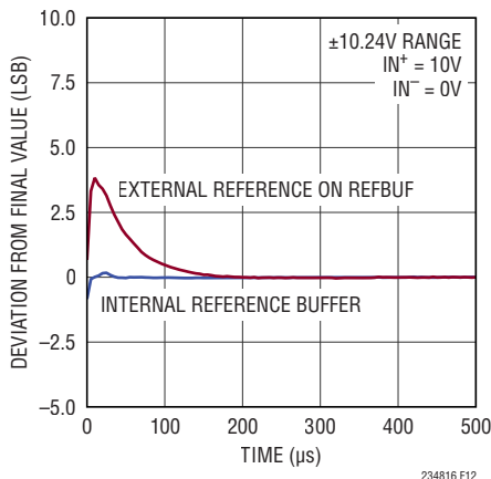
Figure 12. Burst Conversion Response of the LTC2348-16, f_{\text{SMPL}} = 200\text{ksps}
