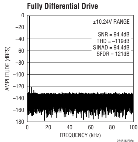
Figure 6c. IN^+/IN^- = -1\text{dBFS} 2kHz Fully Differential Sine, V_{\text{CM}} = 0\text{V} , 32k Point FFT, f_{\text{SAMPL}} = 200\text{kpsps} . Circuit Shown in Figure 6a with LT1469 Amplifiers, R_{\text{FILT}} = 49.9\Omega , C_{\text{FILT}} = 1000\text{pF}
