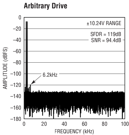
Figure 6b. Two-Tone Test. IN^+ = -7\text{dBFS} 2kHz Sine, IN^- = -7\text{dBFS} 3.1kHz Sine, 32k Point FFT, f_{\text{SAMPL}} = 200\text{kpsps} . Circuit Shown in Figure 6a with LT1469 Amplifiers, R_{\text{FILT}} = 49.9\Omega , C_{\text{FILT}} = 1000\text{pF}
