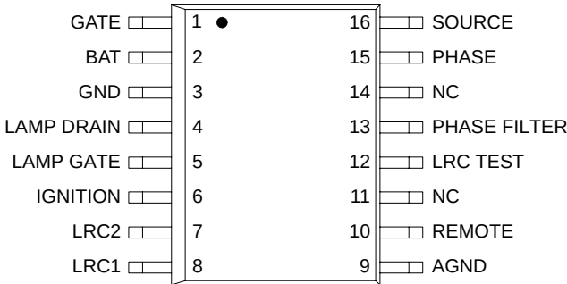
Figure 3. 33099 Pin Connections
