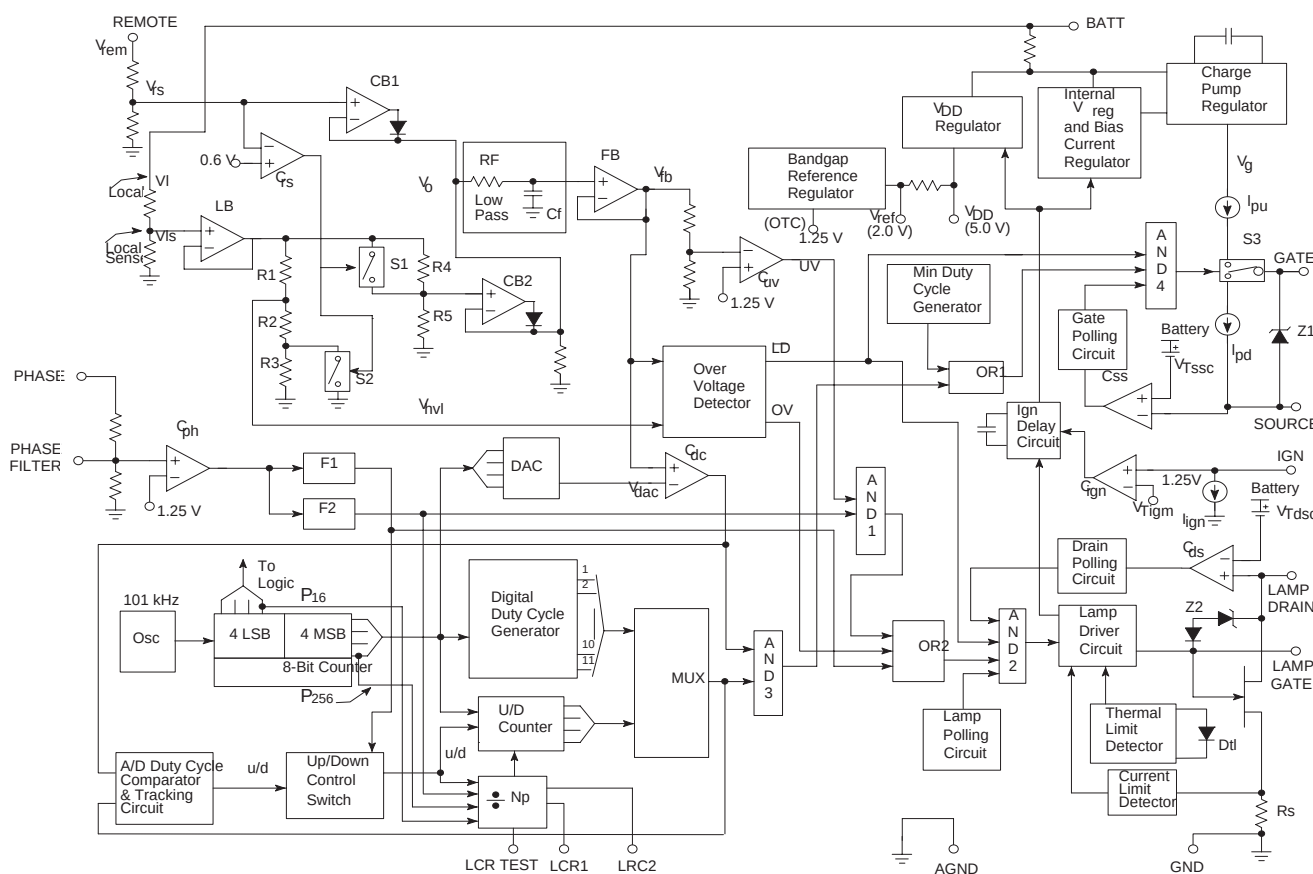
Figure 4. 33099 Simplified Application
