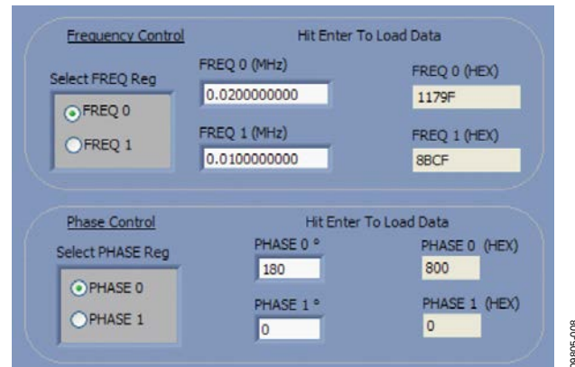
Figure 8. Frequency and Phase Load
