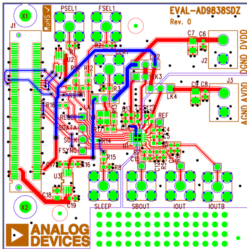
EVAL-AD9838SDZ (Rev. 0) – Component Side View
