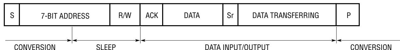
Figure 6. Conversion Sequence
