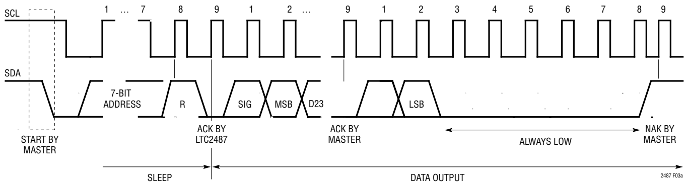
Figure 3a. Timing Diagram for Reading from the LTC2487
