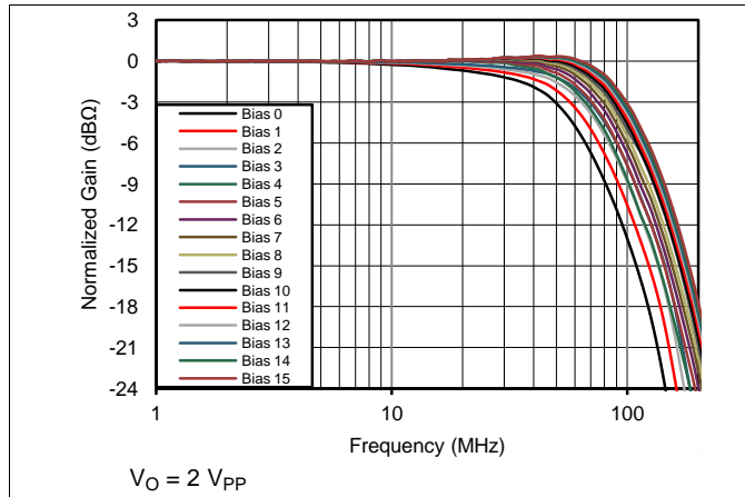
Figure 2. Normalized Small-Signal Frequency Response
