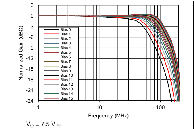
Figure 3. Normalized Large-Signal Frequency Response
