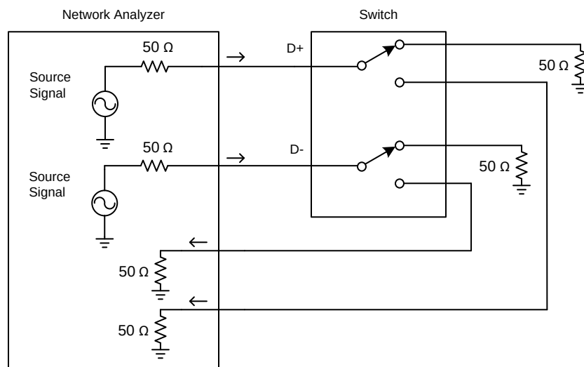
Figure 7. Off Isolation
