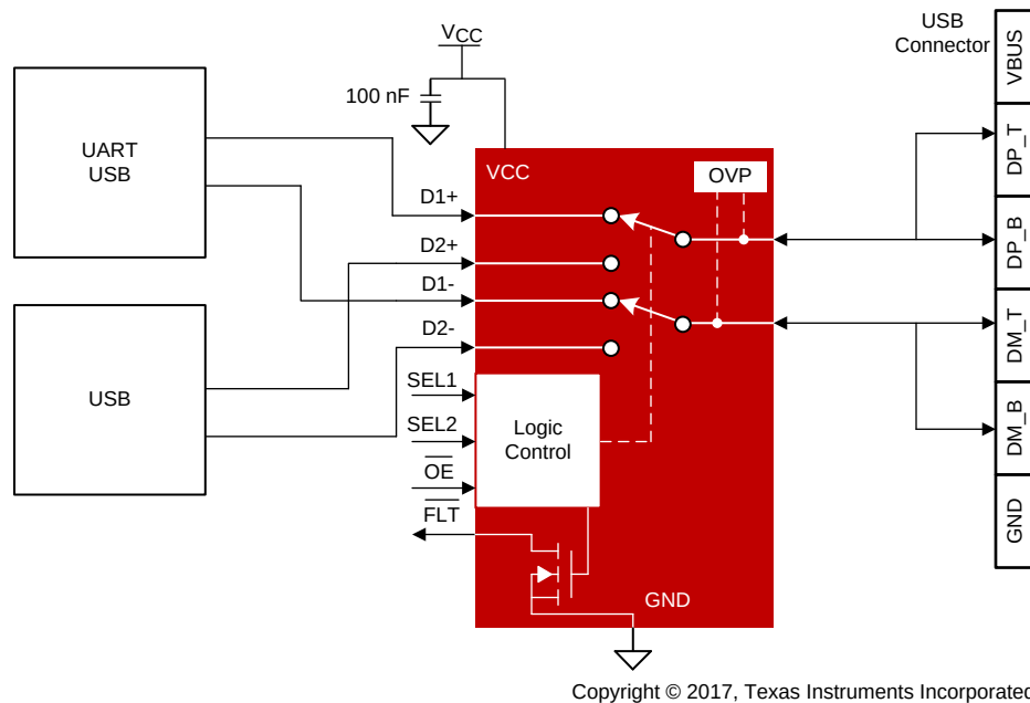
Figure 17. Typical TS5USBC402 Application
