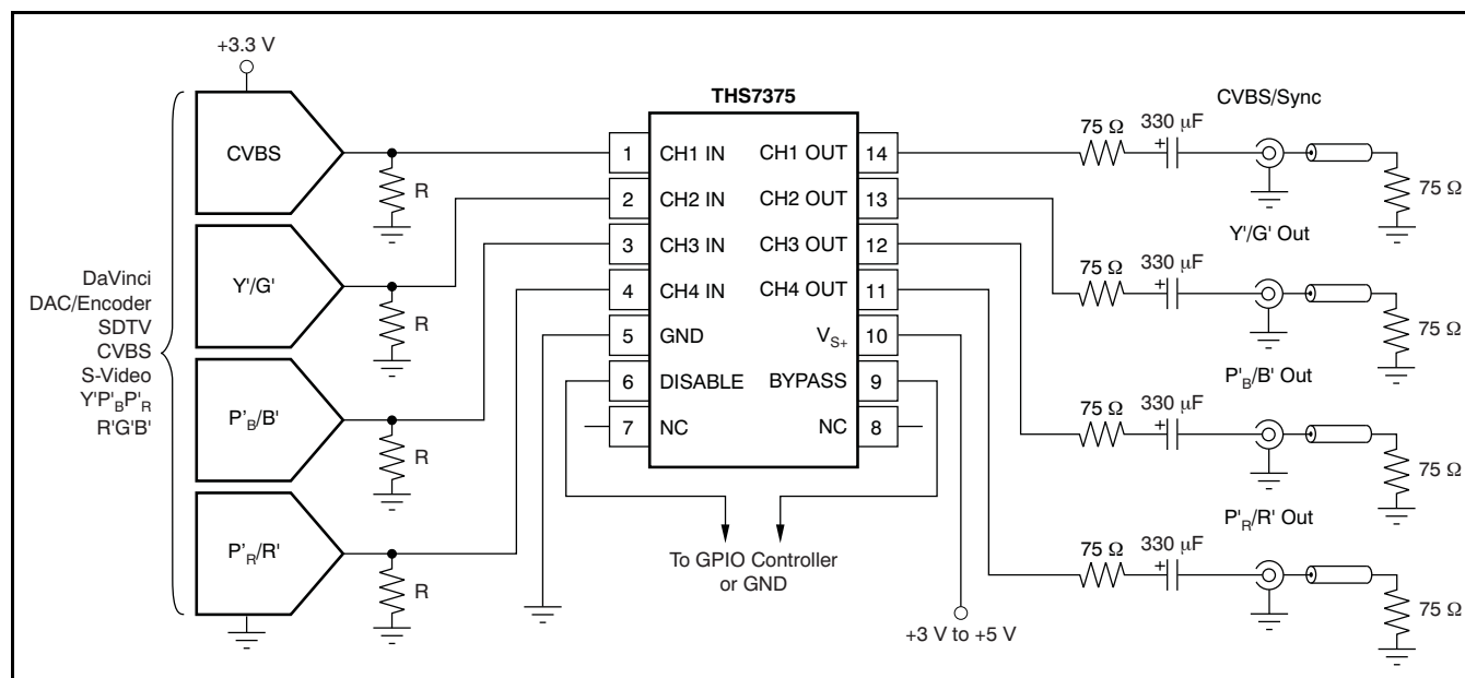
Figure 48. Typical SDTV CVBS/ Y'P'_BP'_R Inputs from DC-Coupled Encoder/DAC with AC-Coupled Line Driving
