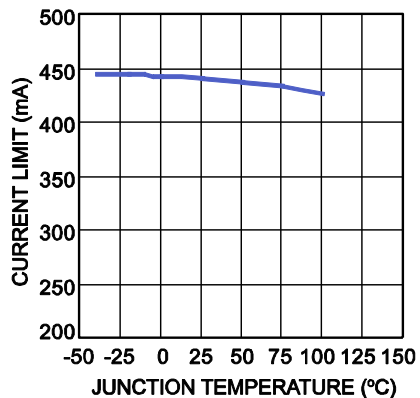
PD Current Limit vs. Temperature
