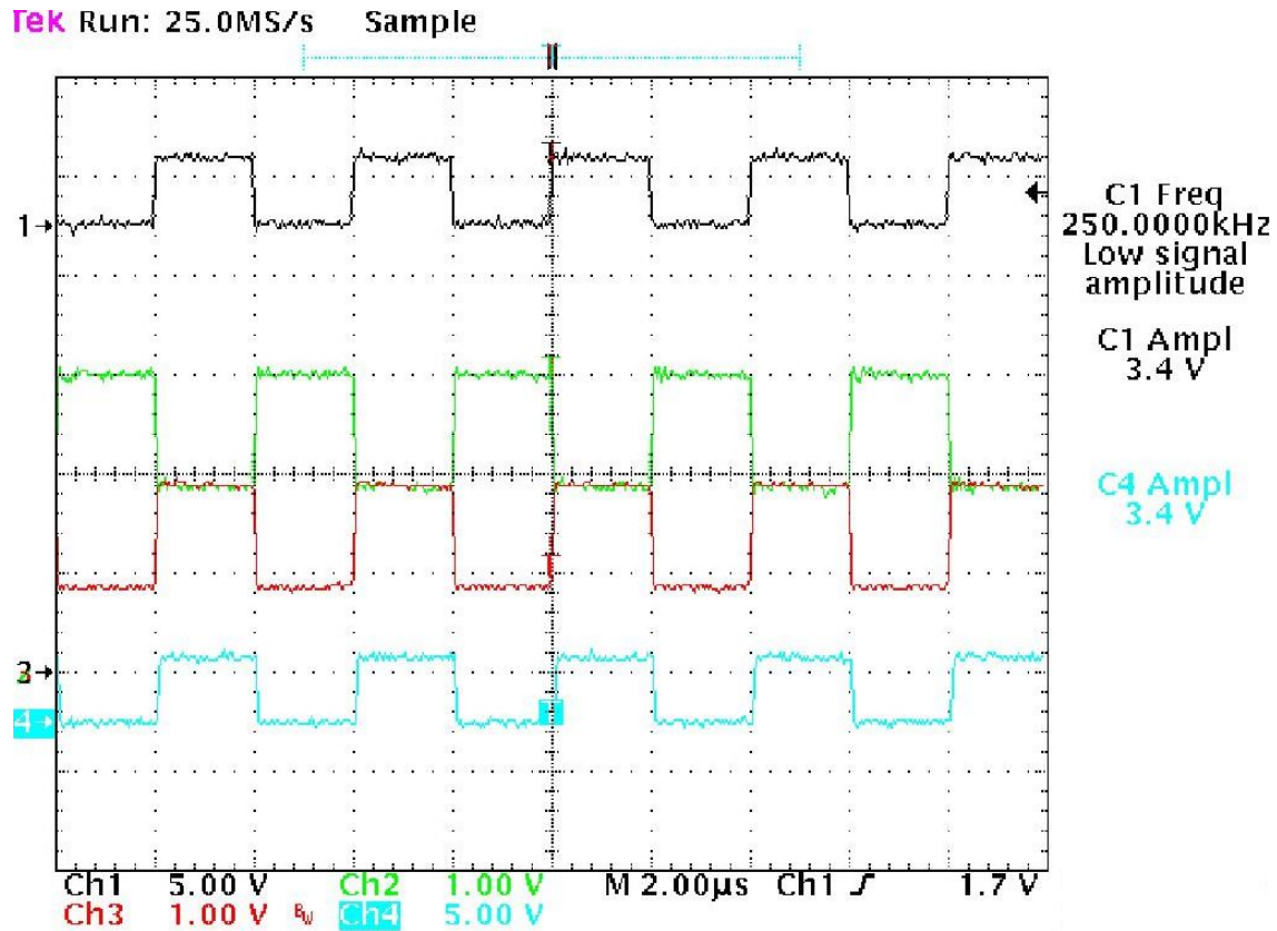
Figure 3. TCAN1043HG-Q1 Normal Operation 500 kbps
