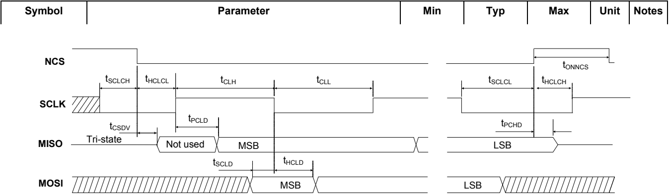
Figure 5. SPI Timing Diagram
