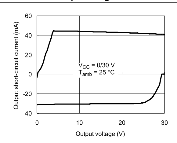
Figure 5. Output short-circuit current vs. output voltage
