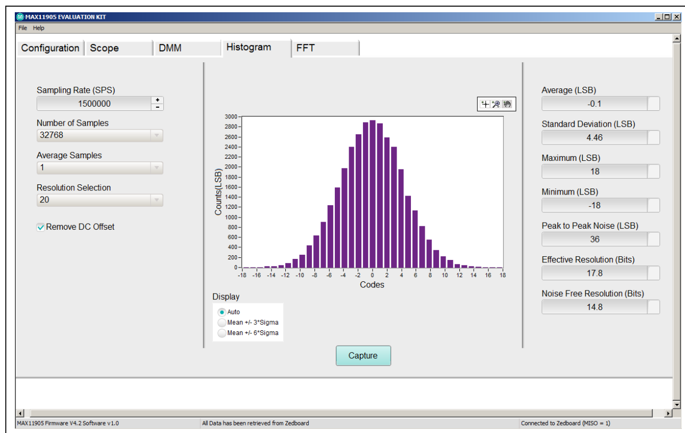
Figure 4. MAX11905 EV Kit Main Window (Histogram Tab)
