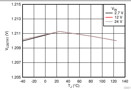
Figure 19. LDSTRT Threshold Voltage vs Temperature
