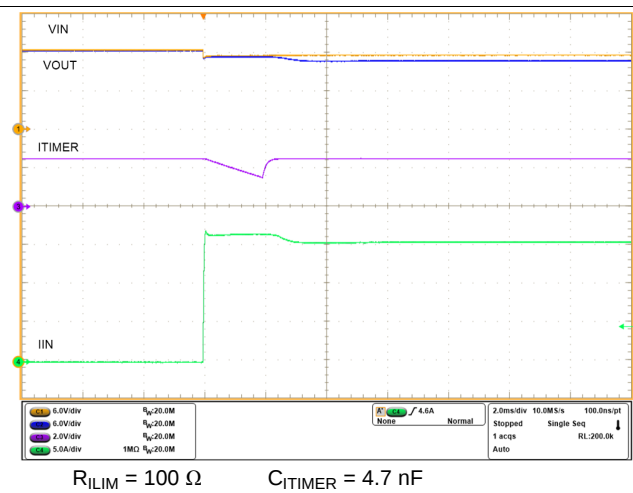
Figure 32. Current Limit With Transient Overcurrent Blanking
