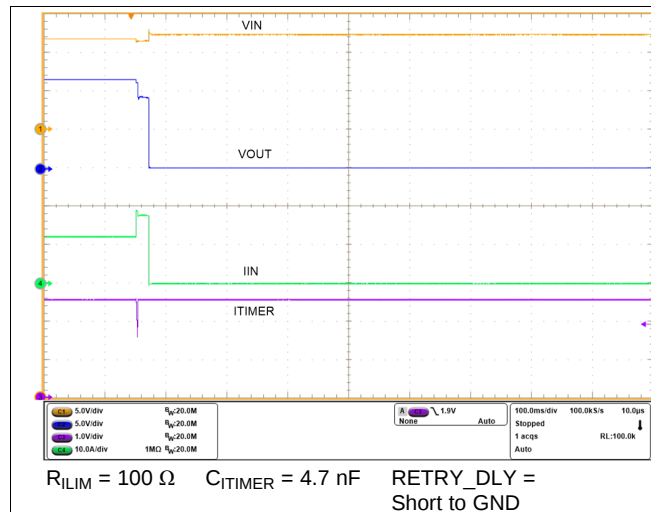
Figure 33. Current Limit Followed By Thermal Shutdown - Latch-off
