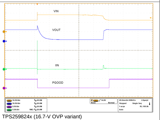
Figure 30. Overvoltage Protection
