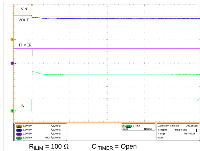
Figure 31. Current Limit Without Transient Overcurrent Blanking
