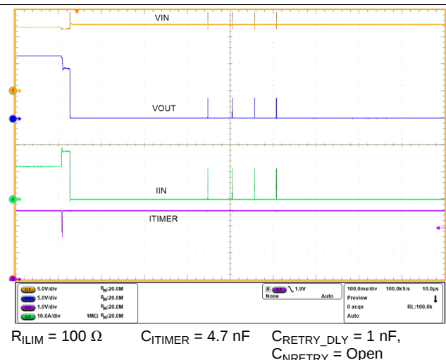
Figure 34. Current Limit Followed By Thermal Shutdown - Auto-Retry
