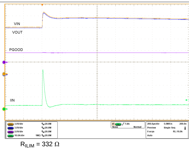
Figure 40. Supply Line Transient Immunity - Input Voltage Step
