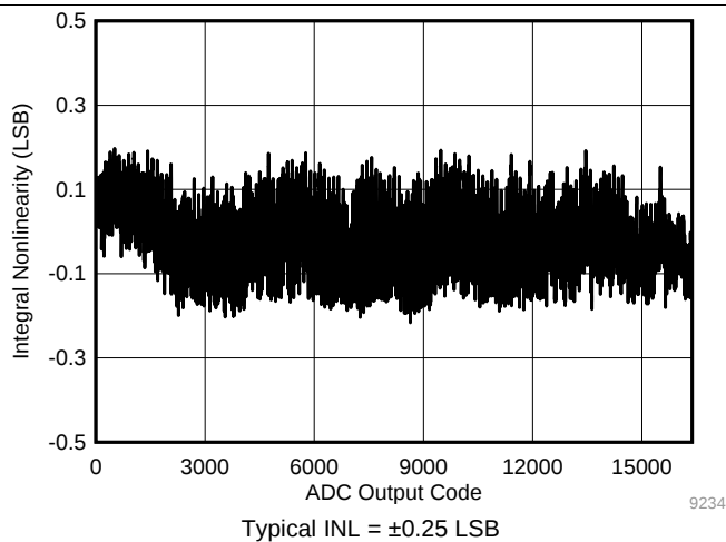
Figure 33. Typical INL
