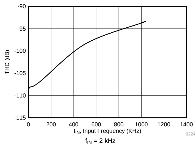
Figure 12. Distortion Performance vs Frequency
