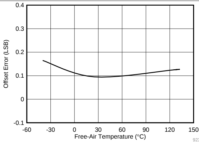
Figure 29. Offset Error vs Temperature
