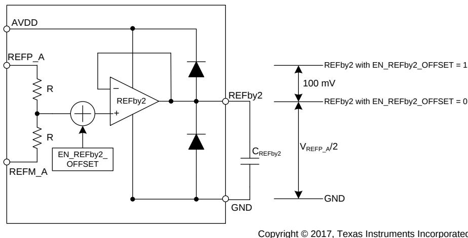
Figure 40. REFby2 Buffer
