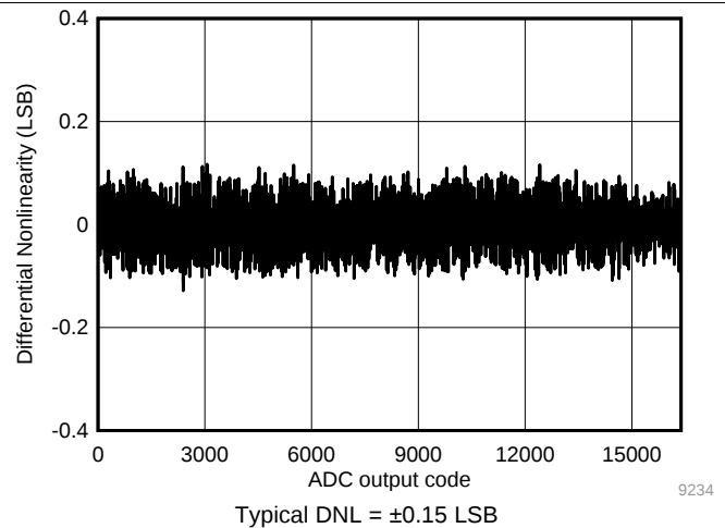
Figure 32. Typical DNL
