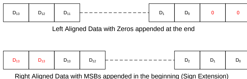
Figure 46. Data Alignment for ADS9234R Devices
