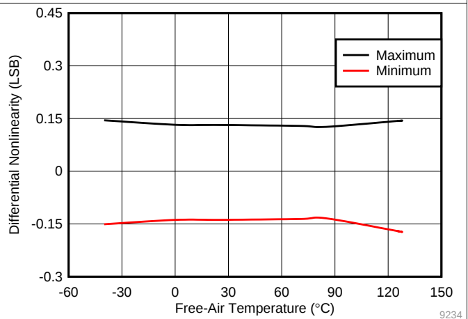
Figure 32. Typical DNL
