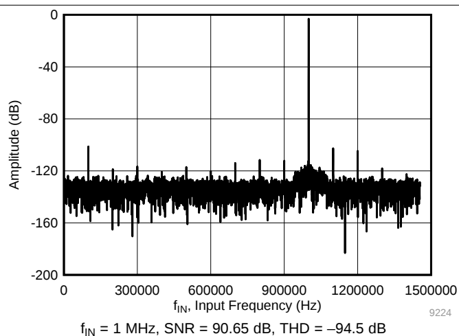
Figure 8. Typical FFT at f_{IN} = 1 \text{ MHz}
