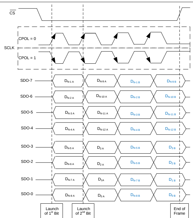
Figure 65. PB-01-AA-SDR and PB-11-AA-SDR Protocols
