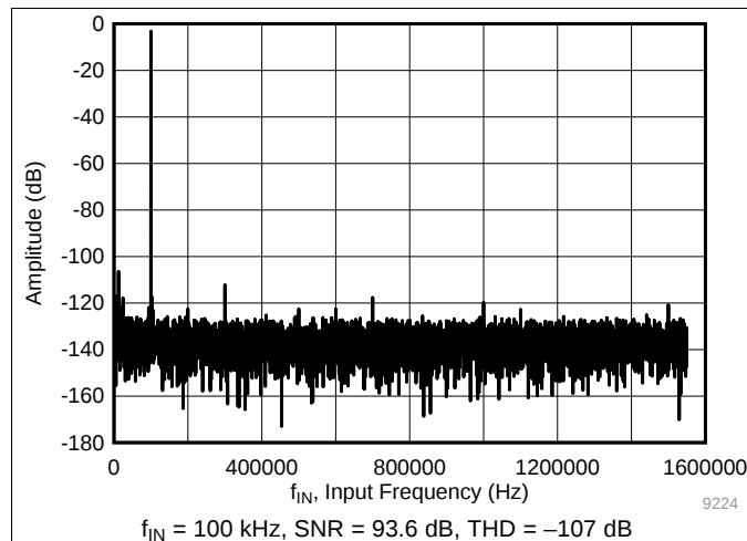
Figure 7. Typical FFT at f_{IN} = 100 \text{ kHz}
