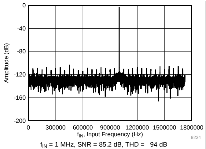
Figure 24. Typical FFT at f_{IN} = 1 \text{ MHz}
