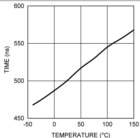
Figure 11. Forced HO Off-time vs Temperature VCCX = 5 V
