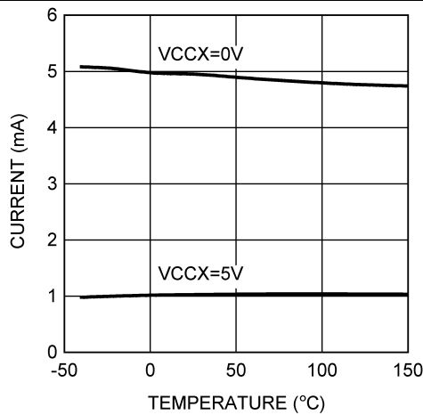
Figure 19. VIN Operating Current vs Temperature
