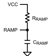
Figure 38. R_{RAMP} to VCC for V_{OUT} > 7.5\text{ V}
