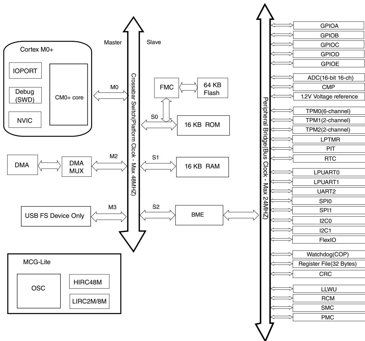
Figure 1. System diagram
