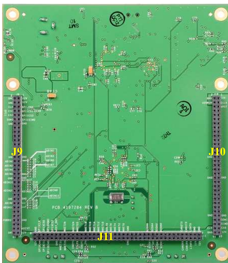
Figure 2-6. J9, J10 and J11 Connectors
