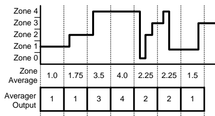
Figure 28. Averager Calculation
