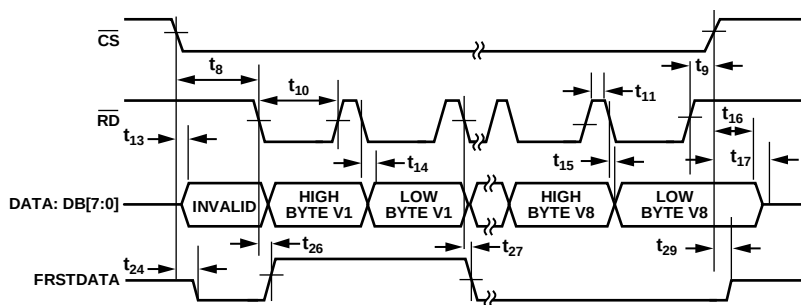
Figure 7. BYTE Mode Read Operation
