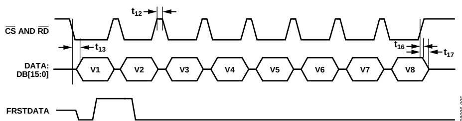
Figure 5. Linked Parallel Mode, \overline{CS} and \overline{RD}
