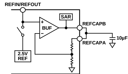
Figure 36. Reference Circuitry
