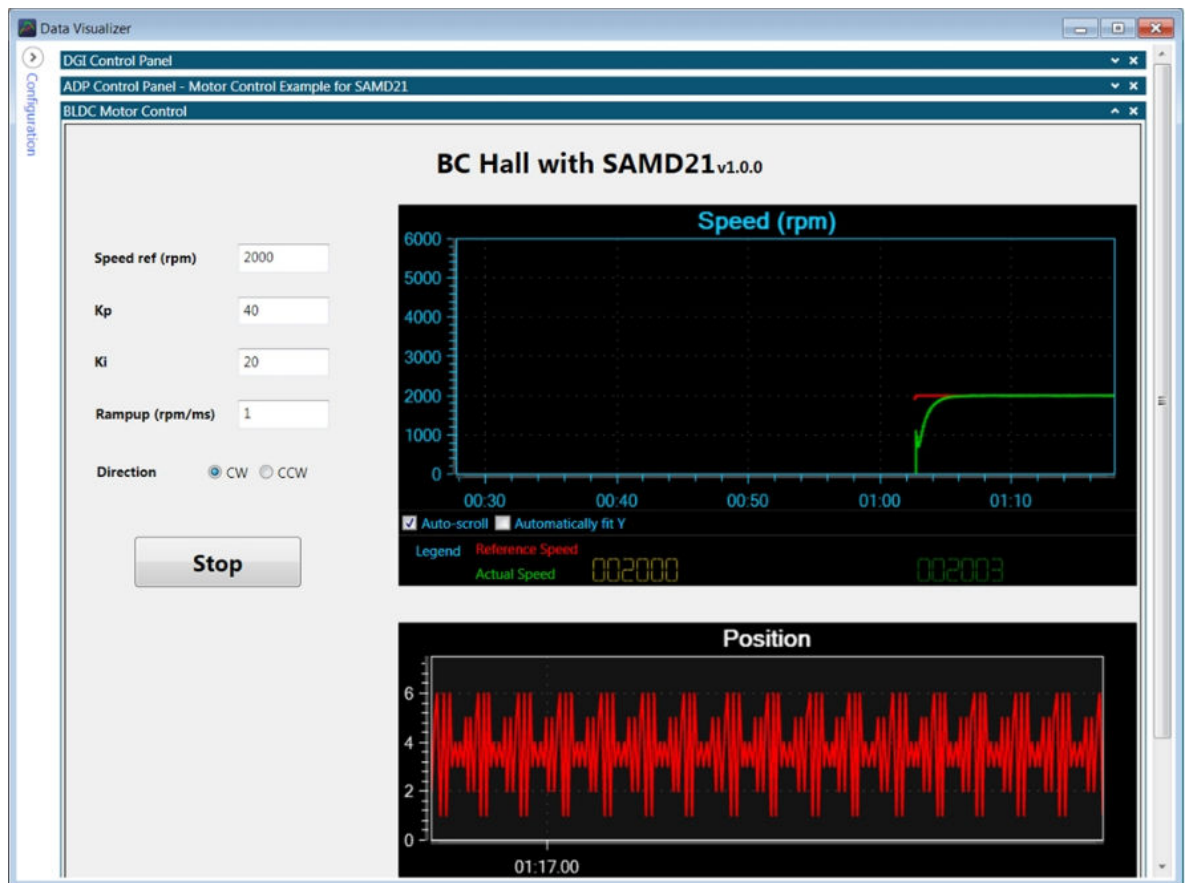
Figure 2-4. Data Visualizer "Start Motor" Window
